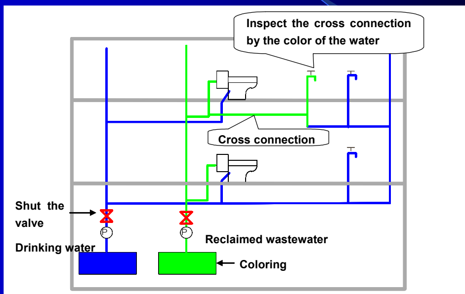
Example of method for confirming cross connection
