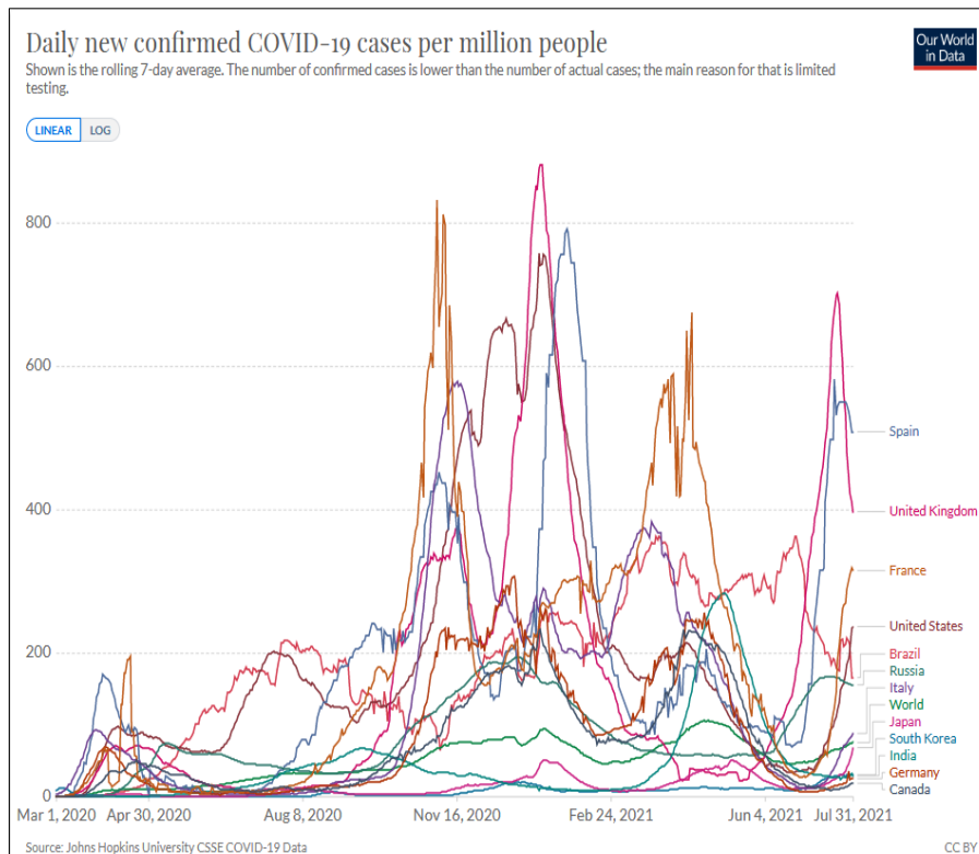
Number of new cases per 1 million population (7-day moving average)
